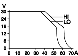
Current limit 1200S24
